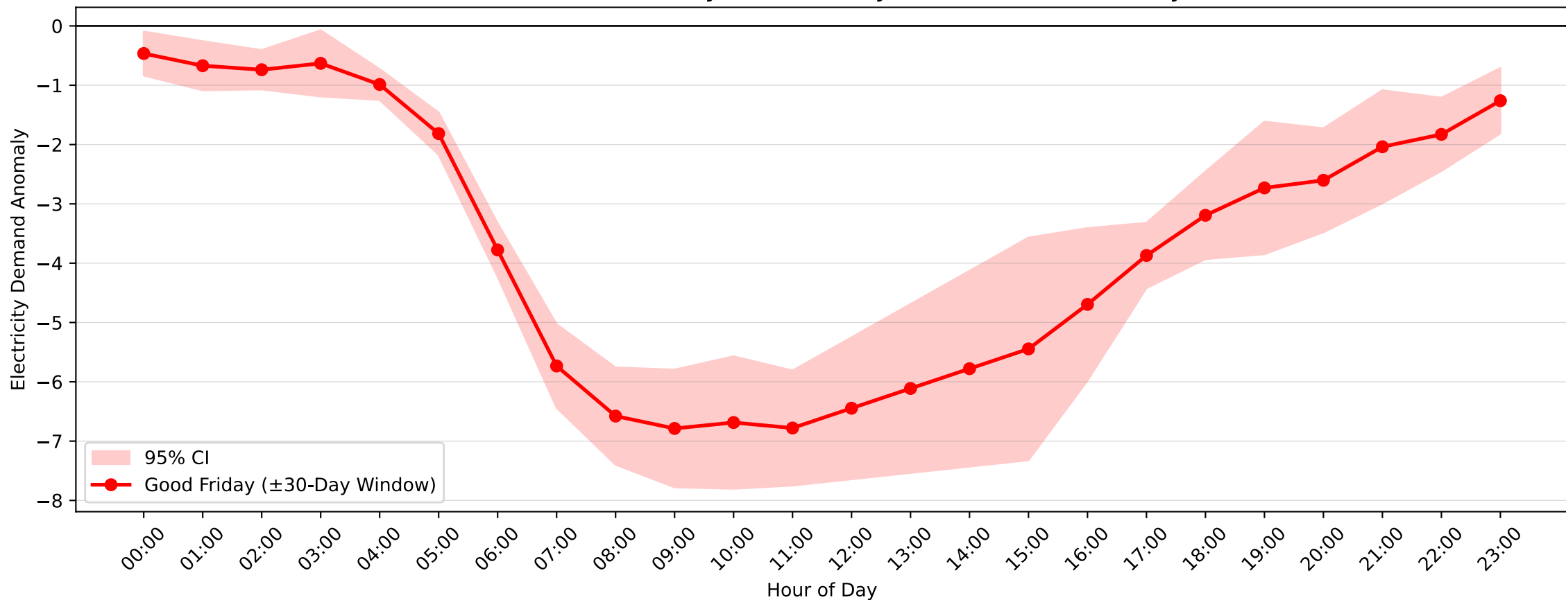
Bankstown Demand Anomaly: Good Friday (2011–2012, \pm 30 -Day Window)
