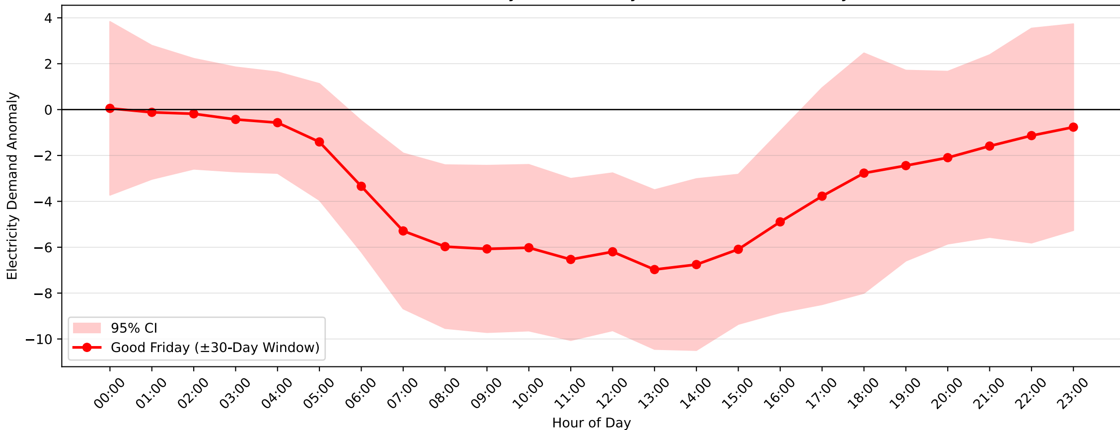
Bankstown Demand Anomaly: Good Friday (2013-2014, \pm 30 -Day Window)
